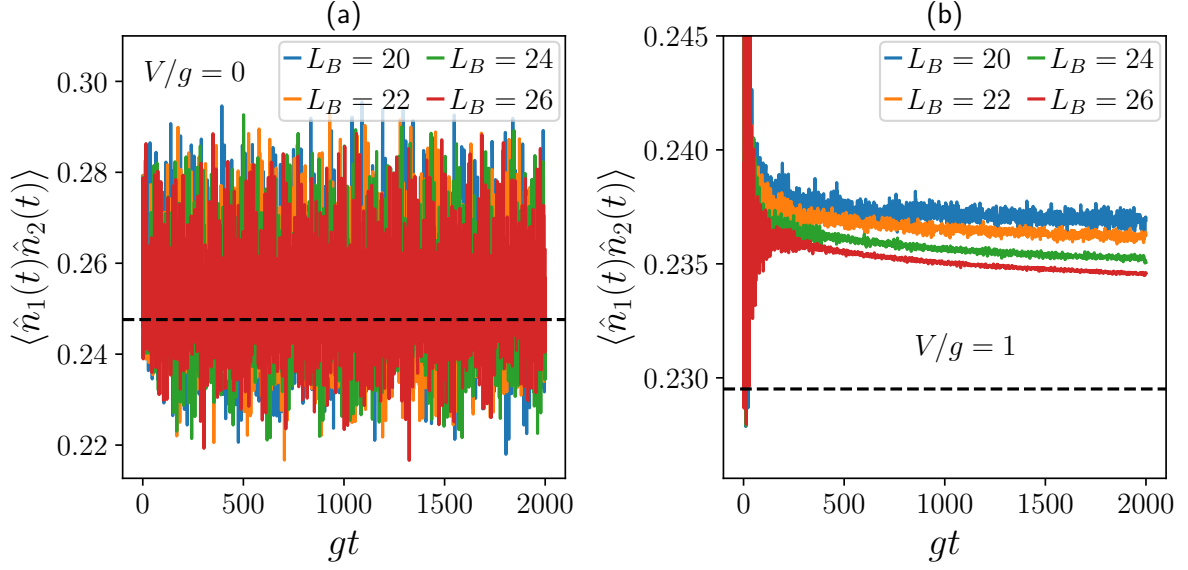
Figure 5: Thermalization in the IQS regime: Plots of the dynamics of the representative DQD observable \langle \hat{n}_1(t) \hat{n}_2(t) \rangle , starting from a randomly chosen initial state (29) of the DQD. In contrast to Fig. 2, where we considered maximal times up to gt_{\text{oqs}} \sim 5 - 8 , we now consider times gt up to 2000, including the regime t \gg t_{\text{oqs}} . Panel (a) shows the free, integrable, DQD case V = 0 . Oscillations are found to persist for all times and for all the chosen values of L_B . Panel (b) shows the dynamics in the interacting, non-integrable* case V = g . The large oscillations disappear after some time gt \sim 400 and only small fluctuations about a relaxed value persist. Those small fluctuations diminish rapidly with increasing bath size L_B . Other parameters: \beta g = 0.1 , \gamma = g , g_B = 2g .
