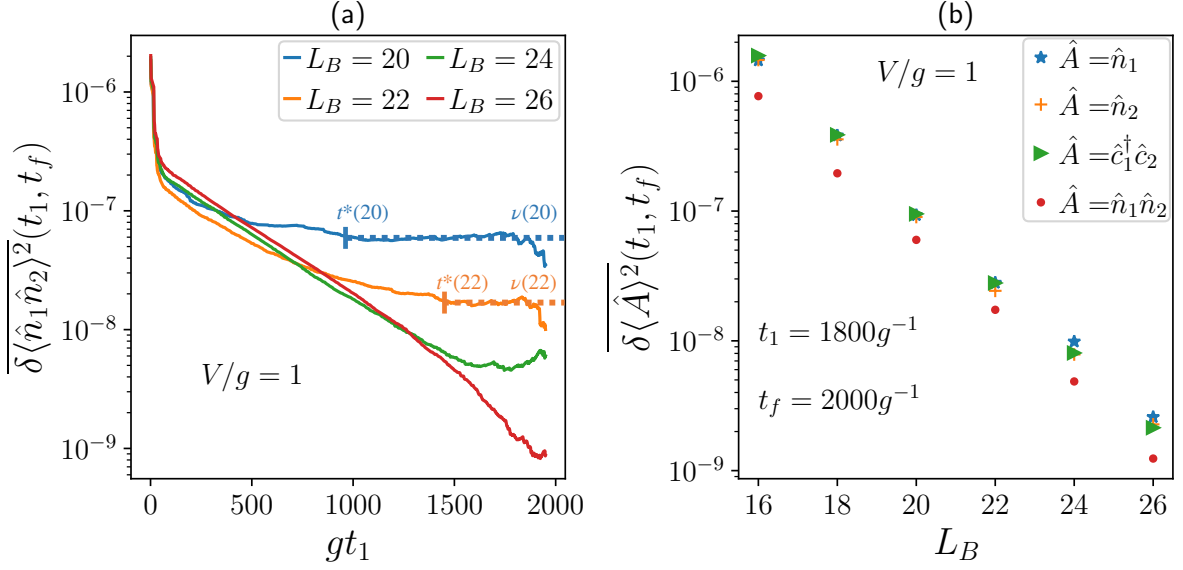
Figure 6: IQS thermalization of interacting DQD with variable bath size L_B : (a) Log-plot of the variance \delta\langle\hat{n}_1\hat{n}_2\rangle^2(t_1, t_f) of data points shown in Fig. 5(b), as a function of initial interval time t_1 , while keeping the final interval time fixed, gt_f = 2000 . Here t_1 is varied between 0 \leq t_1 \leq 1900g^{-1} . Different colours indicate results for various bath sizes L_B . After a time t^*(L_B) , the dynamics reaches an approximately constant value which we call v(L_B) (horizontal dashed lines). The spacing between these saturation values is equal as L_B varies over the values L_B = 20, 22, 24, 26 , which indicates exponential decay of v(L_B) with L_B . (b) Log-plot of the long-time variance \delta\langle\hat{A}\rangle^2(t_1, t_f) for each of the four observables \hat{A} of the interacting DQD, as a function of L_B . The times t_1, t_f are taken large, so that the variance has reached the approximately constant value (c.f. panel (a)). The quantities \delta\langle\hat{A}\rangle^2(t_1, t_f) are numerically evaluated via Eq. (43) with t_1 = 1800g^{-1} and t_f = 2000g^{-1} . The plots show that the variance of each observable \hat{A} decays exponentially with L_B , in line with Eq. (44). Other parameters: V = g, \beta g = 0.1, \gamma = g, g_B = 2g .
