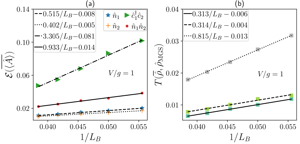
Figure 7: Decaying deviations from full thermalization in the IQS regime: (a) Relative deviation \mathcal{E}(\langle \hat{A} \rangle) , see Eq. (45), of operator expectation values from their mean force Gibbs state (thermal) values as function of 1/L_B , for all four DQD operators. Linear fits (dashed, dotted, dash-dotted, solid) show excellent consistency with (19), for all four operators (25). (b) Trace distance T between the time averaged density matrix \bar{\rho} and the mean force Gibbs state \hat{\rho}_{\text{MGS}} as a function of 1/L_B , for three randomly chosen initial states of the DQD (gray, light green, dark green squares). Linear fits (dotted, dashed, solid) show excellent consistency with (19), for all three initial states drawn from (29). Other parameters: \beta g = 0.1 , \gamma = g , g_B = 2g . Time averages are taken between t_1 and t_f as chosen in Fig. 6(b).
