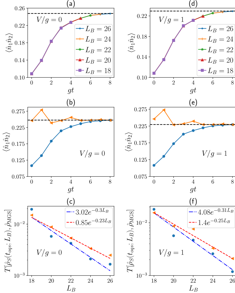
Figure 2: Thermalization in the OQS regime: Panels (a), (b), (c) are for the free fermion case, V = 0 . Panels (d), (e), (f) are for the interacting DQD case with V = g . In panels (a) and (d) we plot the expectation value of a representative observable, \langle \hat{n}_1 \hat{n}_2 \rangle , as a function of time, for different bath sizes L_B , starting from one randomly chosen initial state of the DQD. For each L_B , the time regime t \leq t_{\text{oqs}} is considered, which corresponds to the OQS regime. Plots for larger values of L_B overlap with those of smaller values of L_B but extend to longer times. In panels (b) and (e), we plot the same, but for fixed L_B = 26 and two different randomly chosen initial states (blue and yellow symbols) of the DQD. The horizontal dashed lines in panels (a), (b), (d), (e) show the corresponding expectation value obtained with \hat{\rho}_{\text{MGS}} . In panels (c) and (f), we plot the trace distance between \hat{\rho}_S(t_{\text{oqs}}; L_B) and \hat{\rho}_{\text{MGS}} as a function of bath size L_B for two different choices of initial states (blue and orange symbols) of the DQD. The straight lines (dashed-dotted blue and dashed red) are exponential fits to the symbols, with numerical fit parameters given. Other parameters: g_B = 2g , \gamma = g , \beta g = 0.1 , L_0 = 8 .
