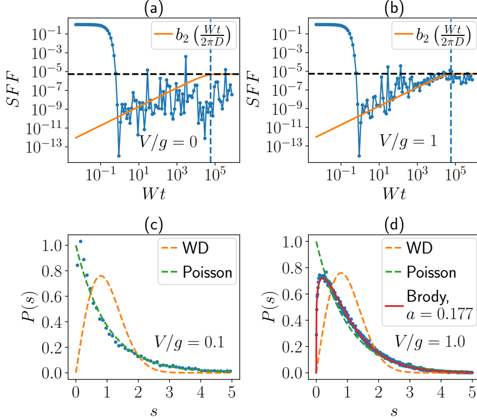
Figure 3: Checking integrability of the interacting DQD: The spectral form factor (SFF) (36) of the full Hamiltonian \hat{H} in (1) is plotted (blue symbols) as a function of Wt , with W = E_{\max} - E_{\min} , for the non-interacting DQD case V = 0 in panel (a), and for the interacting DQD case with V/g = 1 in panel (b). The function b_2 (orange line) is the universal expression given in Eq. (37). The SFF in panel (a) does not approach the function b_2 , while in panel (b), after an initial dip, the SFF oscillates around b_2 , evidencing the SFF behaviour expected of a non-integrable model. The vertical dashed line shows the transition point from ramp to plateau, at Wt = 2\pi D , with D = 2^{L_B+2} . The results in (a) and (b) are for L_B = 16 (total chain size L_B + 2 = 18 ). The horizontal dashed line is located at 1/D . Panel (c) shows the system's level-spacing distribution P(s) (blue dots) at V/g = 0.1 (almost free fermion case) for L_B = 16 . It is evident that it is close to the Poissonian distribution P^{\text{Poi}}(s) , (39) (dashed green), as expected for an integrable system. Panel (d) shows the level distribution P(s) for the interacting DQD model at V/g = 1.0 for L_B = 16 . The level-spacing distribution is still far from the Wigner-Dyson (WD) distribution (dashed yellow) expected for fully non-integrable systems. But, P(s) closely follows a Brody distribution (red line) which, unlike the Poisson distribution (dashed green), goes to zero at zero spacing s .
