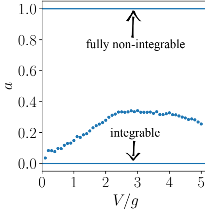
Figure 4: Partial non-integrability of the interacting DQD : The figure shows the values of a , obtained by fitting the level-spacing distribution at half filling of the interaction DQD with the Brody distribution, as a function of interaction strength V . The value a = 0 corresponds to a Poisson distribution, which is expected for integrable systems, while a = 1 corresponds to a Wigner-Dyson distribution, expected for fully non-integrable systems. We see that even on increasing V , a does not approach 1. This evidences non-integrable* behaviour of the interacting DQD. The results are for L_B = 16 (total chain length L_B + 2 = 18 ).
