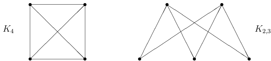
Figure 1.1: The graphs K_4 and K_{2,3} .
