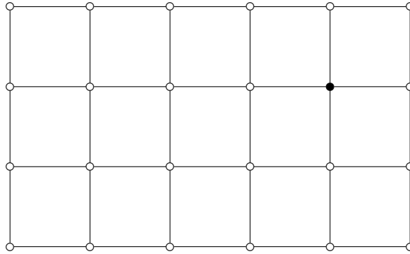
Figure 1.3: An example of grid graph P_4 \square P_6 .
