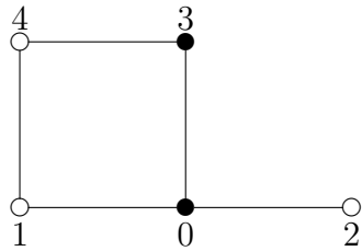
Figure 5.1: A dominating set of \Gamma_3 .
