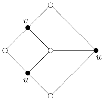
Figure 5.5: Configuration respect to vertices u, v and w .
