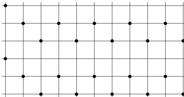
Figure 3.7: The left-over graph (with one cycle) of (C_{3r} \square C_n) - M , where n is odd.
