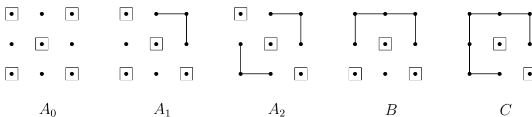
Figure 3.6: The 5 types of vertices in S (the vertex in the center is the vertex that we mean for the type).
