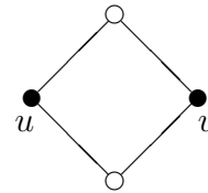
Figure 5.4: u \in C, v \in \bar{C}, v is a Type-2 vertex and u is a Type-2 mate.
