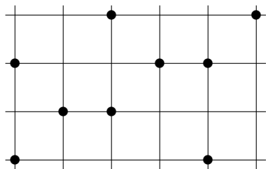
Figure 3.2: A decycling set of C_4 \square C_6
