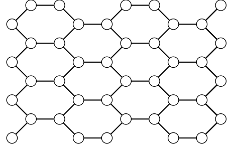
Figure 1.1.3: A portion of the hexagonal grid.
