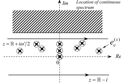
Figure 3: Contour deformation: \int_{\mathbb{R}-i} dz = \sum_{e,s} \int_{\mathcal{C}_e^{(s)}} dz + \int_{\mathbb{R}+i\omega'/2} dz
