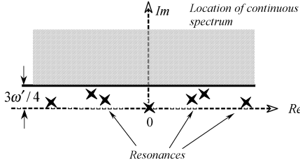
Figure 2: Spectrum of K_\lambda(\omega) . Resonances \varepsilon_e^{(s)} are uncovered.
